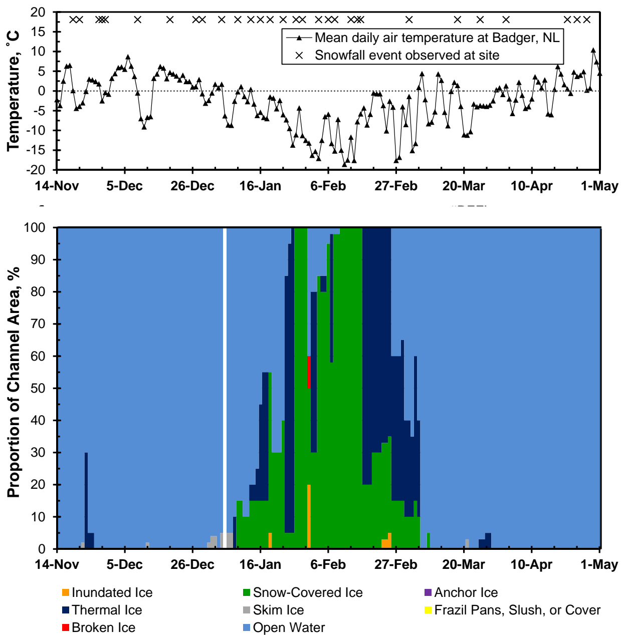
Figure 18. Ice conditions at Compensation Creek (regulated) downstream site for winter 2010-2011 (cameras H5 and M4). Data gaps are denoted by white spaces.
