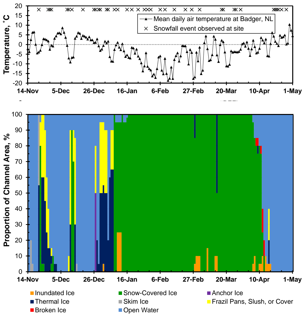
Figure 22. Ice conditions at No Name Creek (unregulated) downstream site for winter 2010-2011 (cameras R4 and M6).
