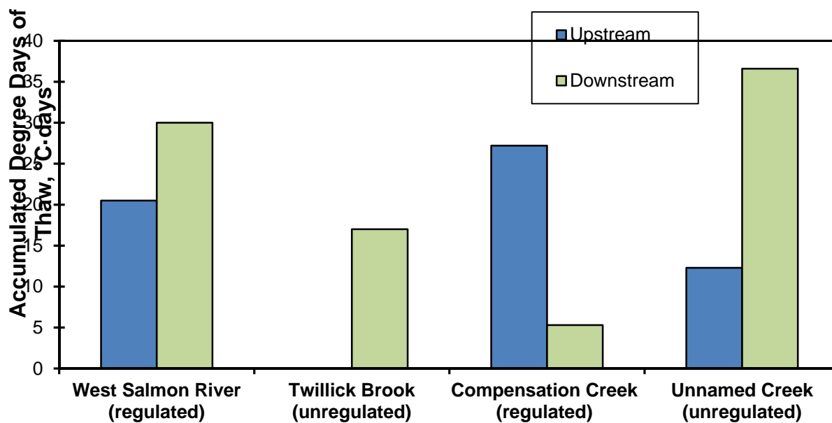
Figure 26. Accumulated degree days of thaw at Badger, NL when streams are first ice free.
