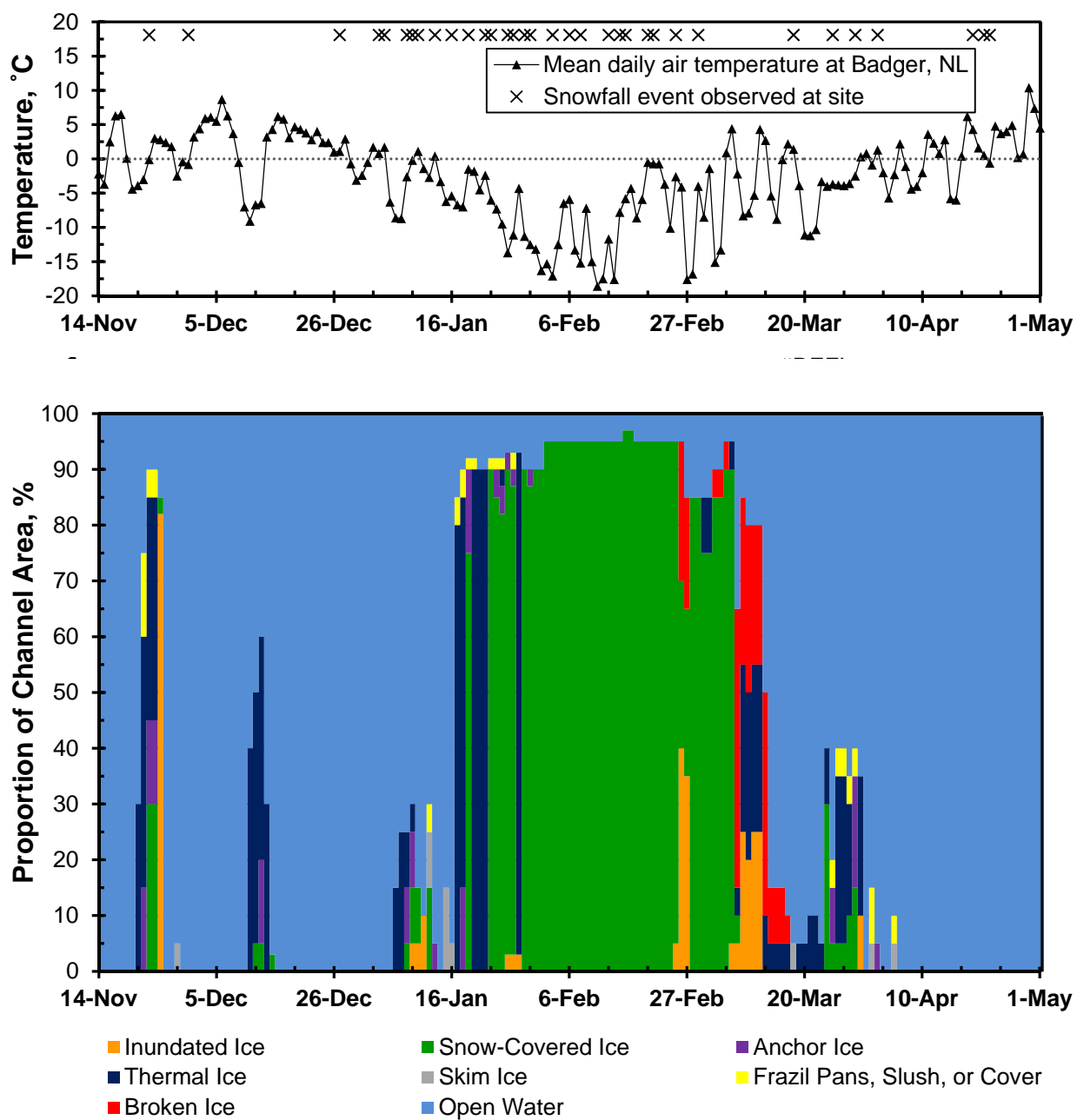
Figure 12. Ice conditions at Twillick Brook (unregulated) downstream site for winter 2010-2011 (cameras H3 and M7).
