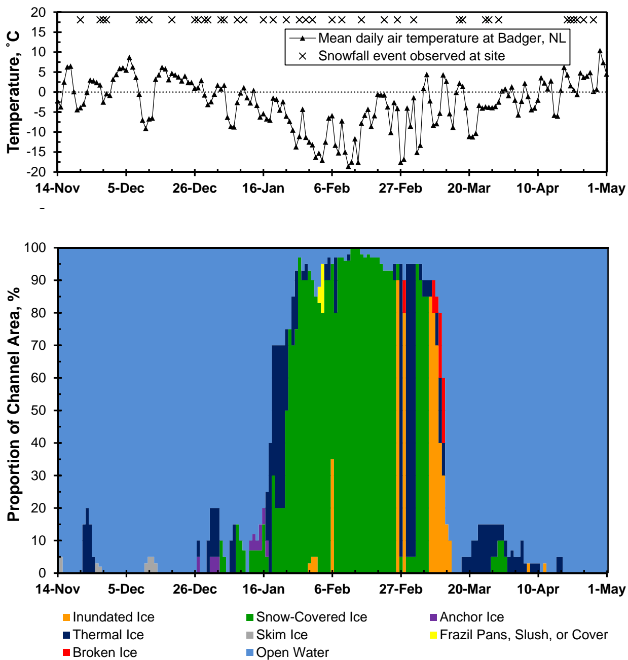
Figure 20. Ice conditions at No Name Creek (unregulated) upstream site for winter 2010-2011 (cameras H4 and M8).
