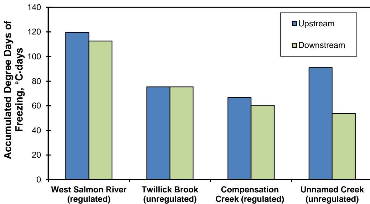
Figure 25. Accumulated degree days of freezing at Badger, NL when first permanent ice forms at each stream.
