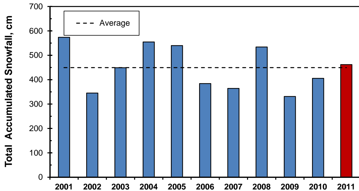
Figure 3. Total accumulated snowfall at Gander, NL.
